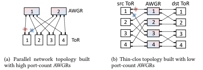
Figure 1: Flat topologies in AWGR-based optical DCNs.
