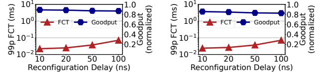
Figure 8: NegotiaToR under various reconfiguration delays at 100% load.
