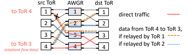
Figure 16: Traffic-aware selective relay on the thin-clos topology. Data relay is enabled for the large volume of data from ToR 4 to ToR 3. When selecting the intermediate ToR, ToR 1 is excluded due to the high volume of direct traffic to ToR 4, which would result in bandwidth competition at ToR 1 → AWGR 3 link. In contrast, ToR 2 can be selected to relay the data, avoiding potential goodput damage.
