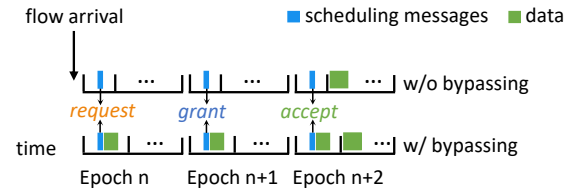
Figure 5: Bypassing scheduling delay with unscheduled transmission in the predefined phase.
